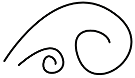
WIND
