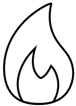
FIRE
