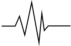
EARTHQUAKE
