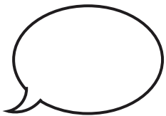
GENTLE WHISPER
