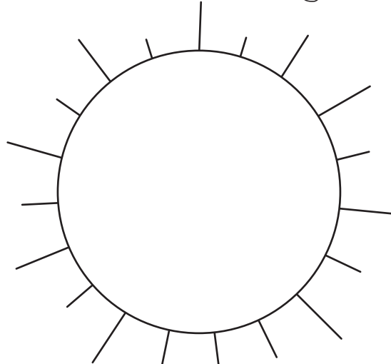
MERCURY
