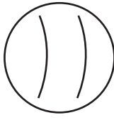
NEPTUNE
